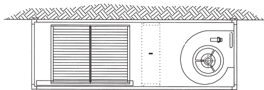
ARRANGEMENT (H)
